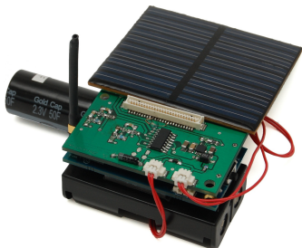
Fig. 1. Energy Harvesting Platform for the IRIS node
